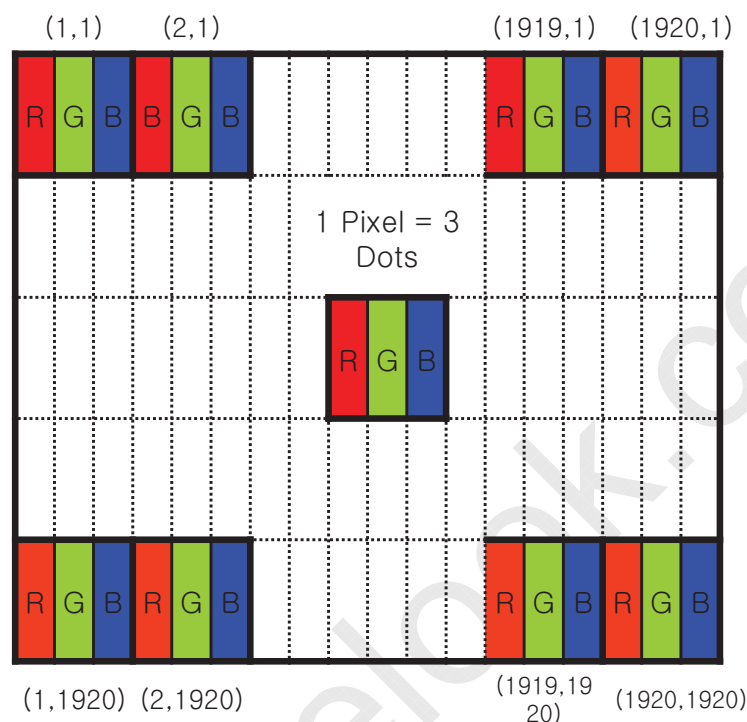
Display Position of Input Data (V-H)
