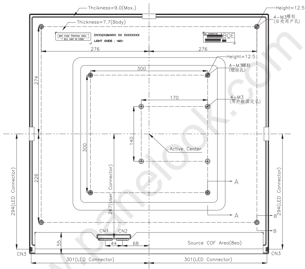
Figure 6. TFT-LCD Module Outline Dimensions (Rear view)
