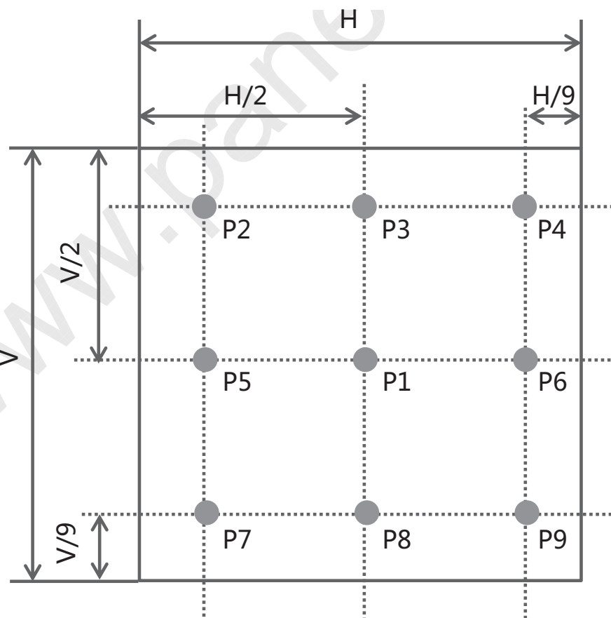
Figure 2. White Luminance and Uniformity Measurement Locations (9 points)
