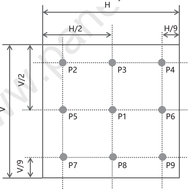
Figure 2. White Luminance and Uniformity Measurement Locations (9 points)
