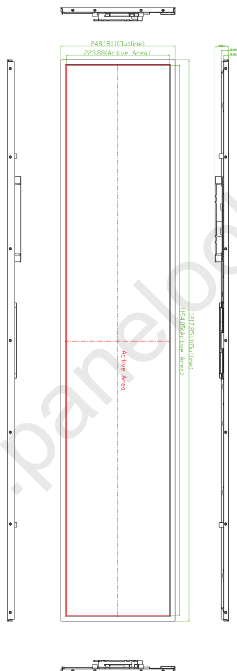
Figure 5. TFT-LCD Module Outline Dimensions (Front view)
